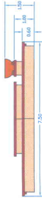
CENTER COLUMN PLANTBOX #1
